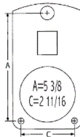
Axle Hole Spacing
